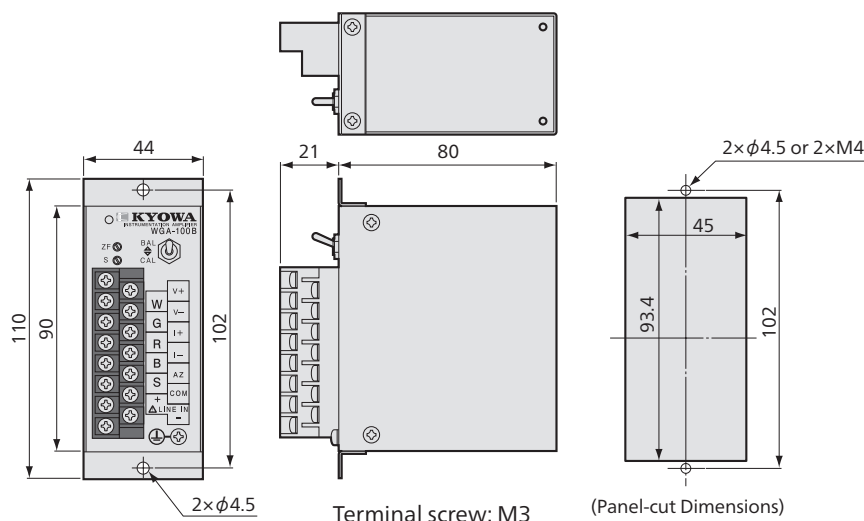
DIN rail mounting fixture included
